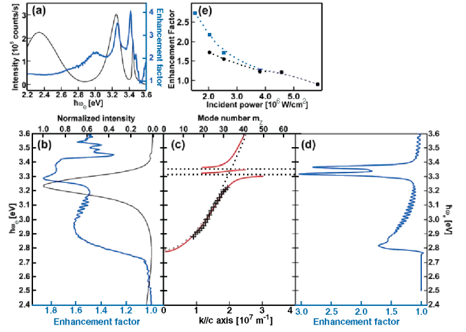
FIG. 2 (color). (a) Average spectrum (black line) and enhancement spectrum (blue line) of a wire excited with \hbar\omega = 1.72 eV, which shows, near the exciton resonances, a peak splitting in the enhancement spectrum of 164 meV. (b) Average spectrum (black line) and enhancement spectrum (blue line) of a wire excited with \hbar\omega = 1.72 eV. The enhancement spectrum shows a peak splitting of 102 meV near the exciton resonances and modulations due to Fabry-Pérot interference in the transparent region (2.7–3.2 eV). (c) Exciton-polariton dispersion (red lines) calculated with Eq. (1) from the resonances of the A (3.309 eV), B (3.315 eV), and C (3.355 eV) excitons (dotted horizontal lines) and a photon mode confined in the nanowire cavity (dotted curve). For clarity, we do not show the strongly damped modes in the anticrossing energy-gap. The crosses indicate the energetic peak positions obtained from the Fabry-Pérot maxima of the enhancement spectrum shown in panel (b). These maxima are equidistantly spaced at m_z^*(\pi/L) in k space ( L = the length of the wire = 5.19 \mu\text{m} ) and give the slope of the exciton-polariton dispersion between 2.7 and 3.2 eV. (d) Calculated enhancement resulting from the dispersion curve shown in (c). (e) Excitation power dependence of the peaks in the enhancement spectrum.
