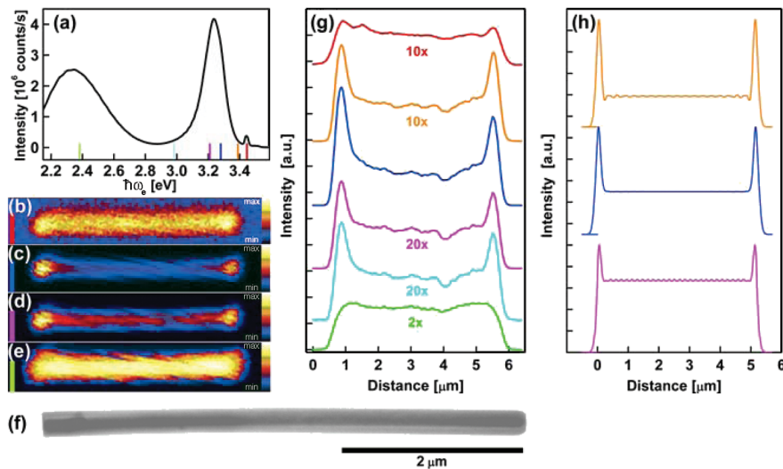
FIG. 1 (color). (a) Average photoluminescence spectrum of a ZnO nanowire for excitation with sub-band-gap light (1.72 eV), showing green and UV photoluminescence as well as second harmonic generation. (b)–(e) Spatially resolved excitation images taken at the emission energies indicated in panel (a) by the colored bars. (f) TEM image of the investigated wire. The wire had a length of 5.19 \mu\text{m} and a diameter of 273 nm. (g) Excitation line traces along the length of the wire ( c axis) at emission energies indicated by the colored bars in panel (a). The profiles are scaled with the indicated factors for clarity. (h) Calculated excitation profiles for the energies shown by the color bars in (a).
